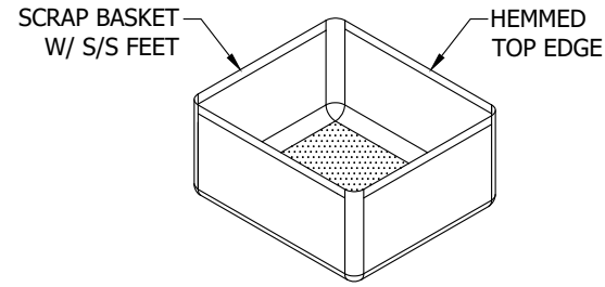
SCRAP BASKET DETAIL
